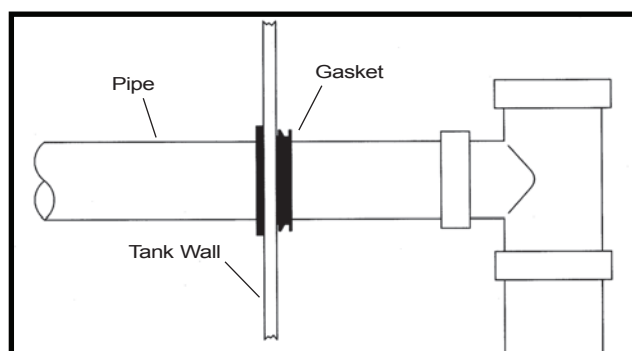
FIG.2 Gasket Detail
