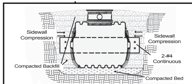
FIG.4 Backfilling
