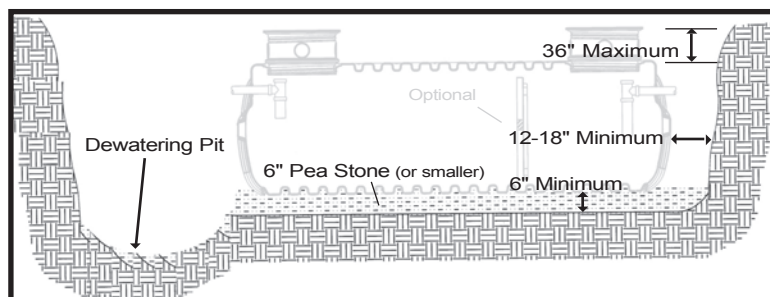
FIG.1 Excavation
